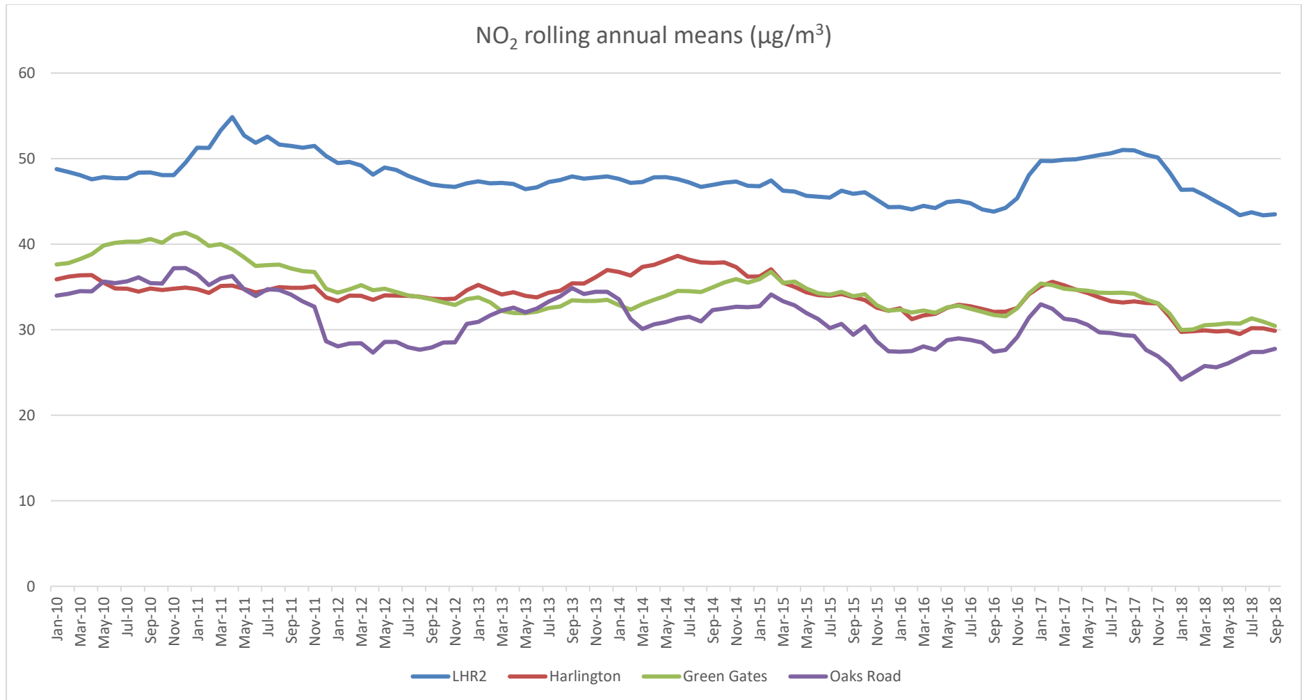
Fig.1. NO 2 rolling annual means at HAL funded sites since 2010 (µg/m 3 )
